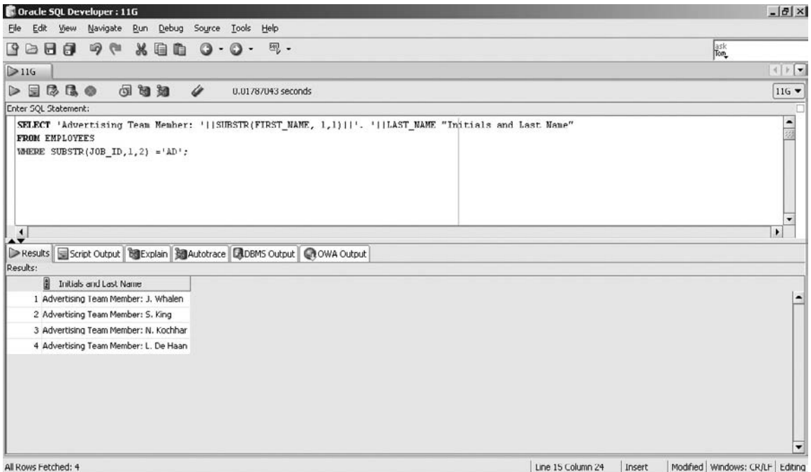
FIGURE 4-11 The SUBSTR function
