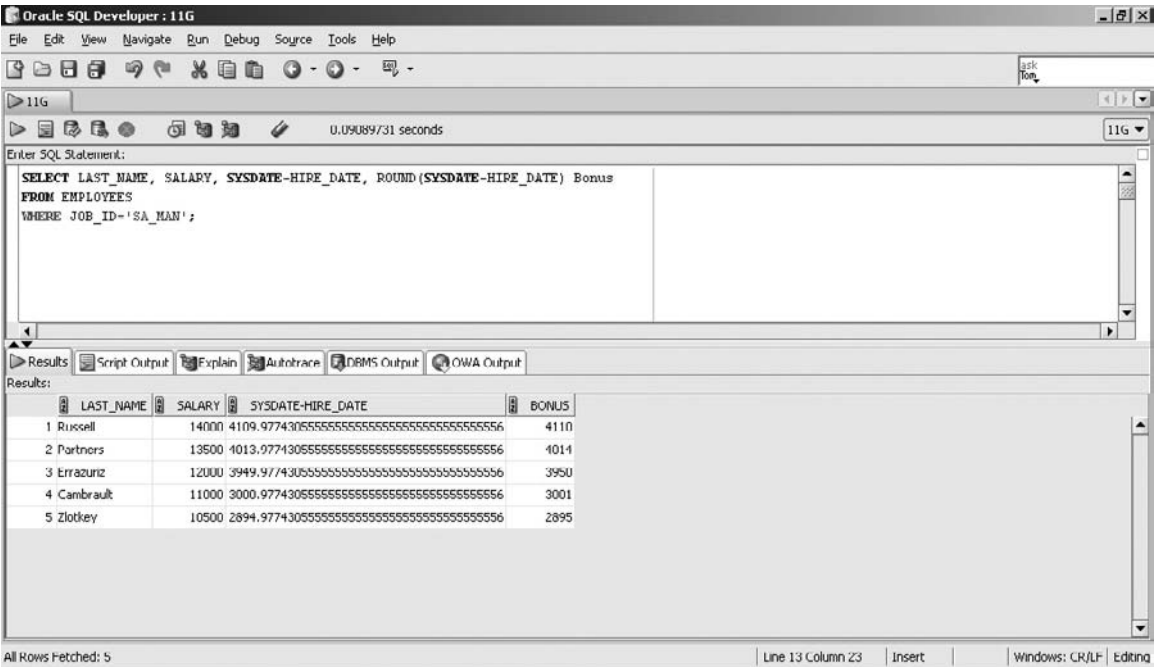
FIGURE 4-13 The numeric ROUND function
