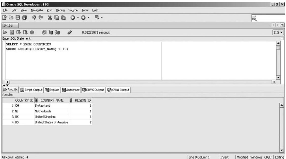
FIGURE 4-7 The LENGTH function
